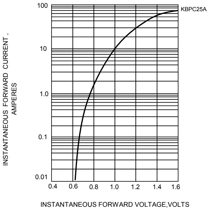
FIG.3-TYPICAL FORWARD CHARACTERISTICS
