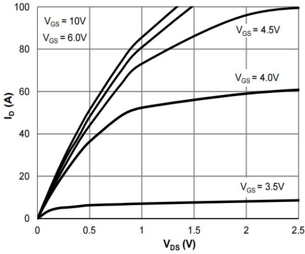
Figure 1: Saturation Characteristics
