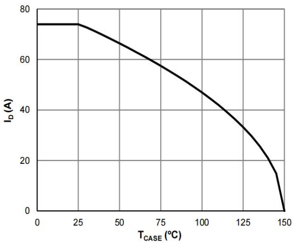
Figure 9: Current De-rating
