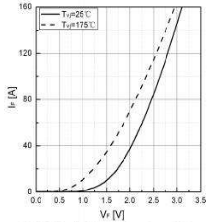
Fig 8. Typical I_F as a function of V_F
