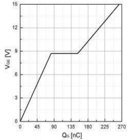
Fig 4. Typical Gate charge
