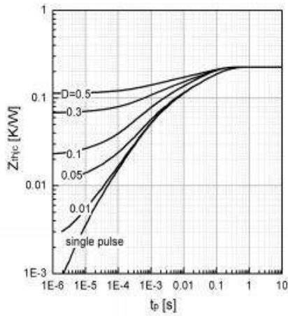
Fig 15. Transient thermal impedance of IGBT
