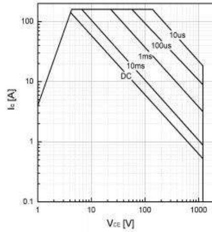
Fig 14. Safe operating area
