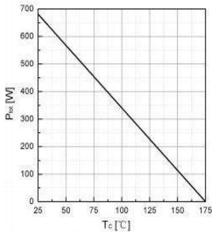
Fig 3. Power dissipation as a function of T_c
