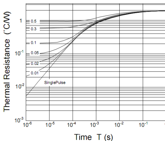
Figure 8. Thermal Impedance
