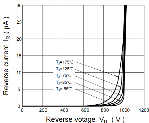
Figure 2. Reverse Characteristics
