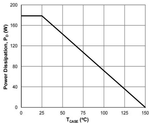
Figure 8: Power De-rating
