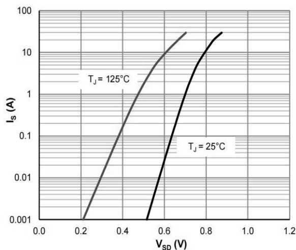
Figure 5: Body-Diode Characteristics
