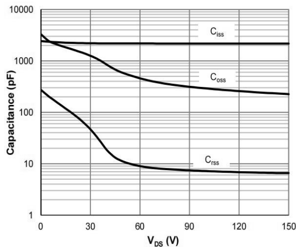
Figure 6: Capacitance Characteristics
