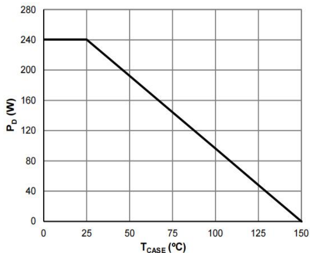
Figure 10: Power De-rating
