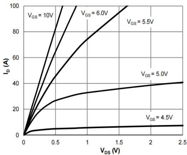
Figure 1: Saturation Characteristics
