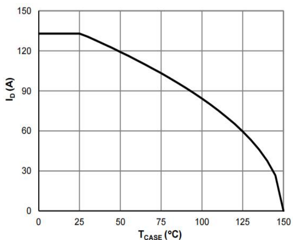
Figure 9: Current De-rating
