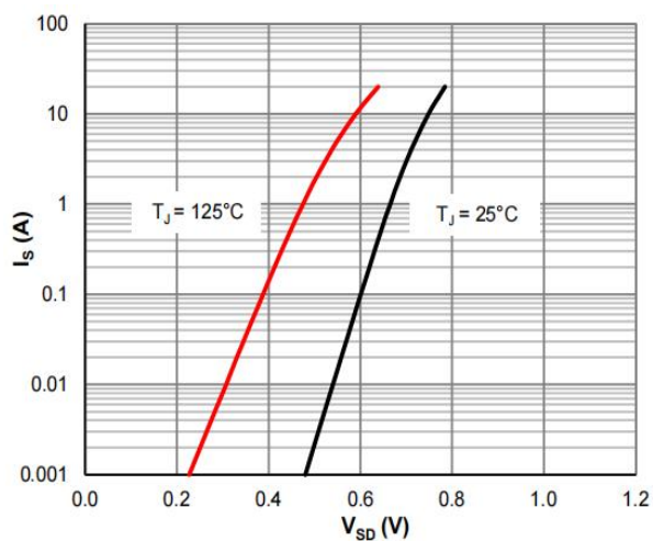
Figure 7: Body-Diode Characteristics
