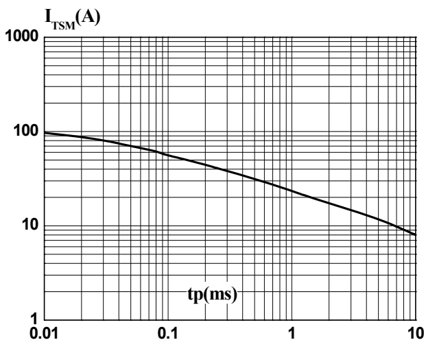
FIG.5: Non-repetitive surge peak on-state current for a sinusoidal pulse with width t_p < 10ms
