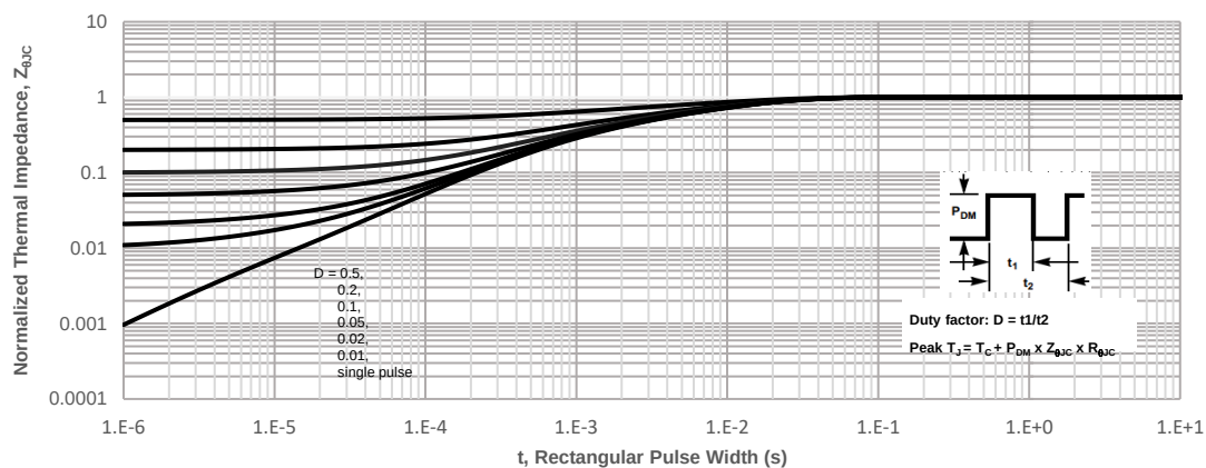
Figure 10: Peak Current Capacity
