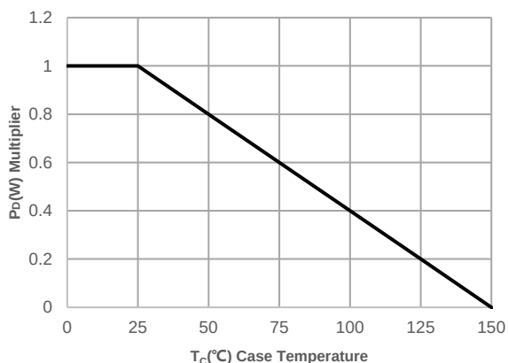
Figure 7: Power De-rating
