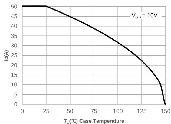
Figure 8: Current De-rating
